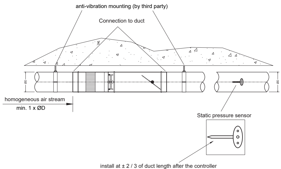
Mounting drawing type AHQ...B
