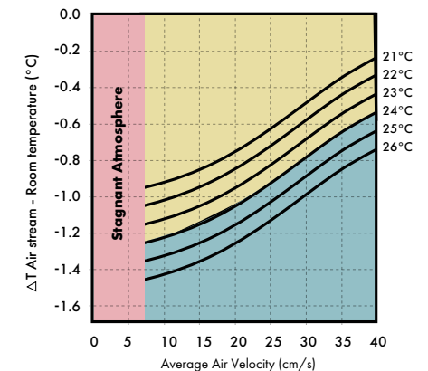
BARCOL-AIR COLMAN COMFORT CHART
