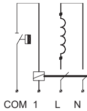
Wiring diagram, 1-stage, 230VAC/1-phase
